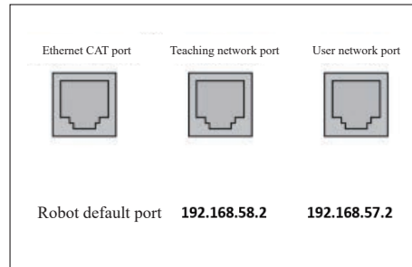
Figure 3 Schematic diagram of the network interface group
